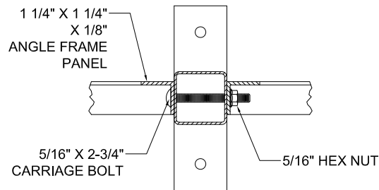
LINE POST CONNECTION
