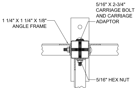
THREE WAY POST
