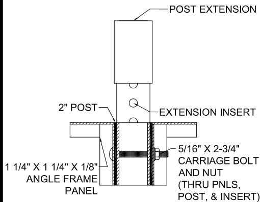
POST EXTENTIONS
