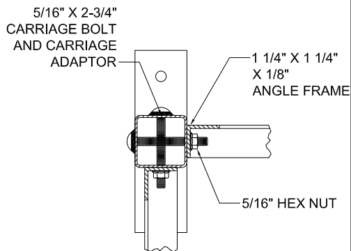
CORNER POST
