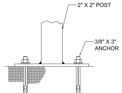
BASE DETAIL
