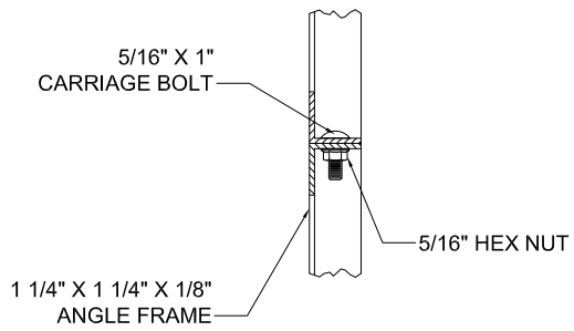
PANEL TO PANEL
