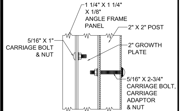
GROWTH PLATE CONNECTION
