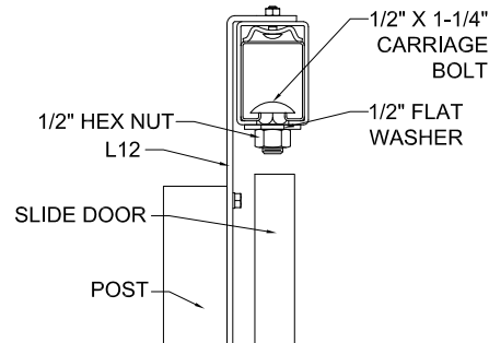
TRACK STOPS
