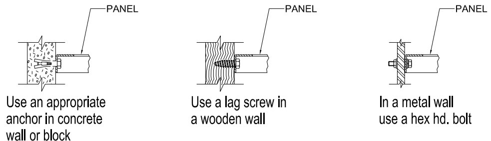
LINE POST CONNECTION
