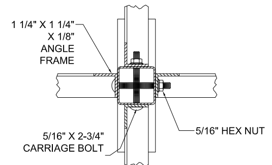
FOUR WAY CONNECTION
