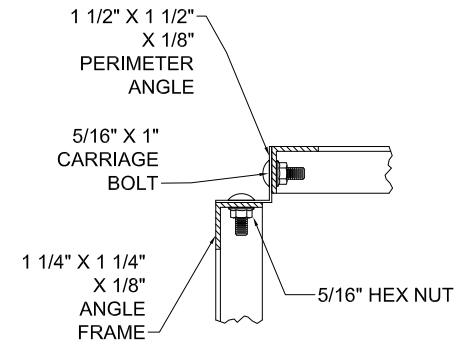
CEILING TO PANEL
