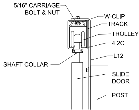
TRACK
